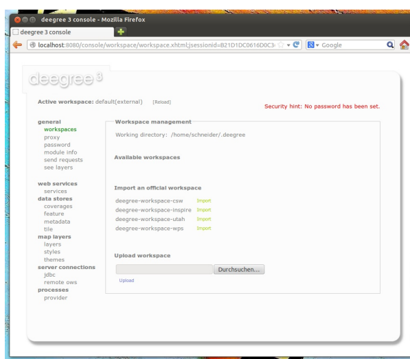
Figure 3.2: Workspaces view
