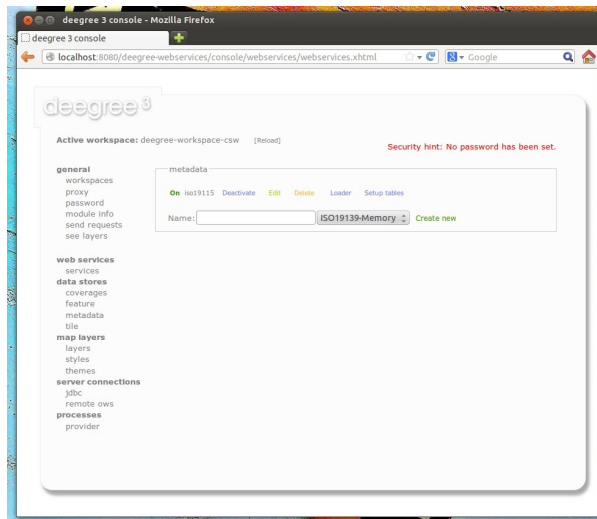
Figure 4.5: Displaying metadata store resources
