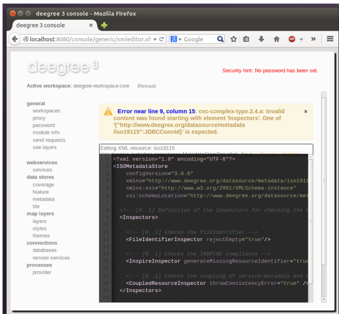
Figure 49. The services console displays an XML syntax error
