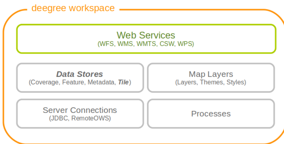
Figure 81. Tile store resources provide access to pre-rendered map tiles
