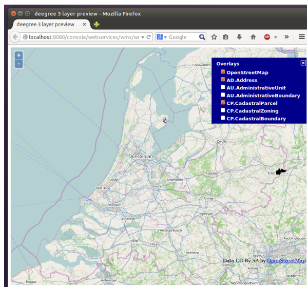
Figure 3.7: Ad.Address layer after insertion of example Address features
