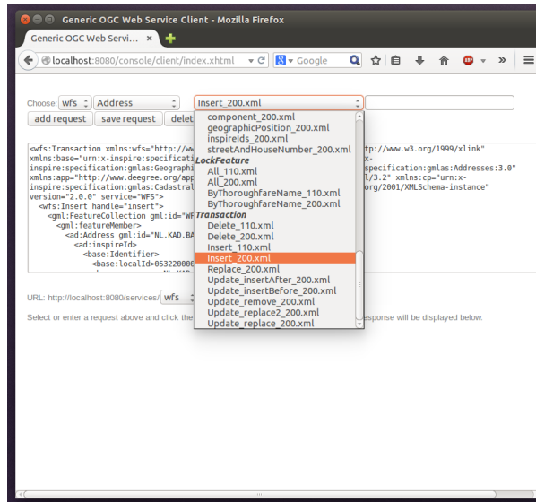
Figure 3.6: WFS-T example requests
