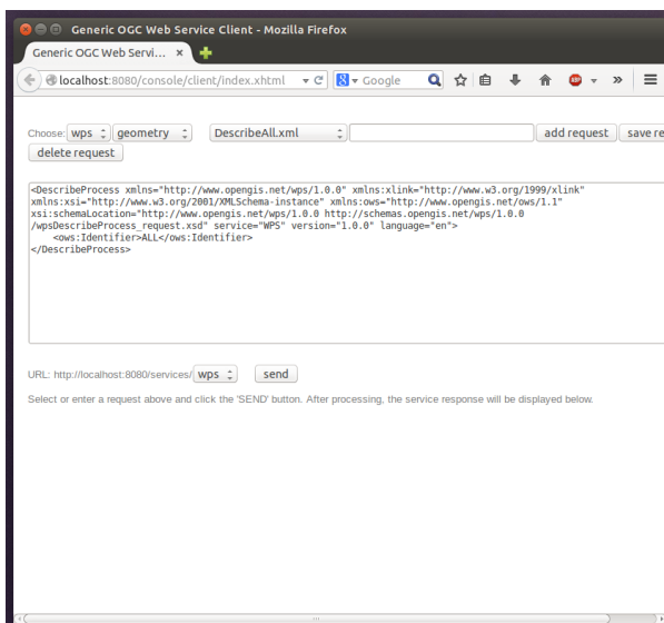
Figure 3.24: Choosing a WPS example request
