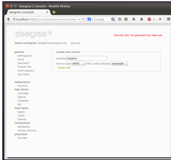
Figure 4.13: Adding a WMS resource with identifier “mywms”
