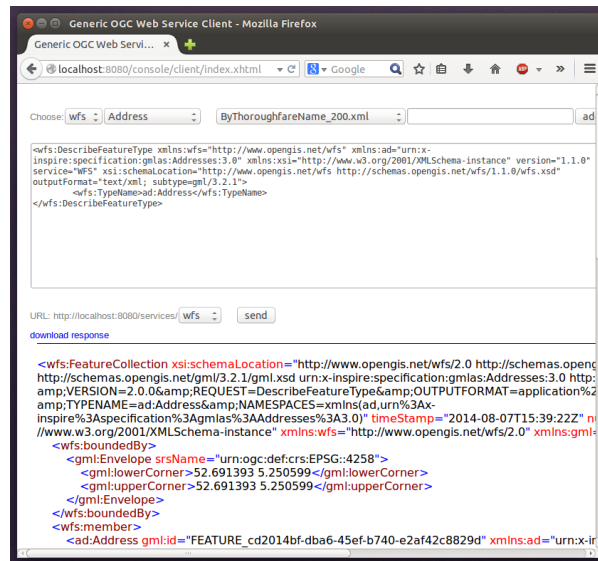
Figure 6.19: More WFS examples
