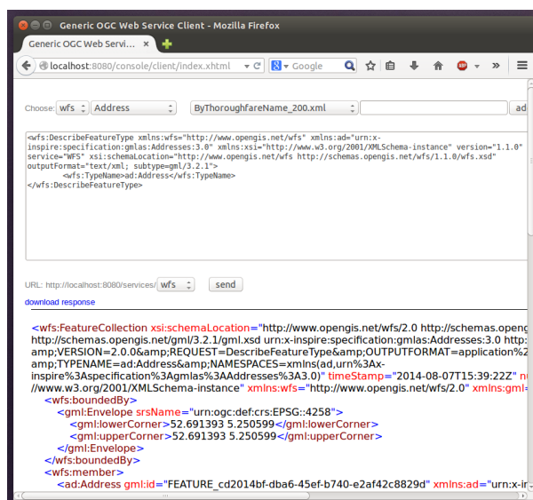
Figure 3.8: WFS query examples
