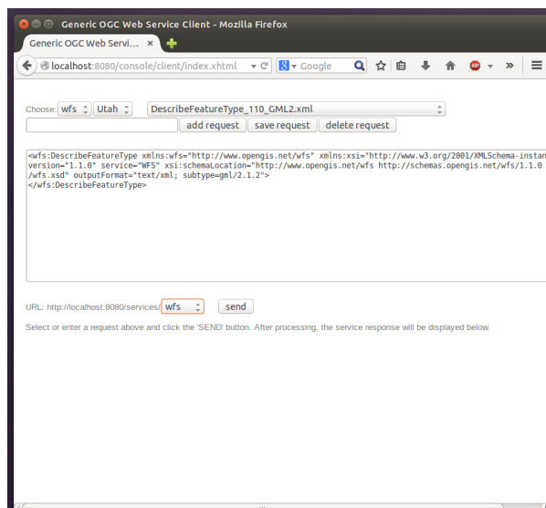
Figure 3.12: Sending example requests
