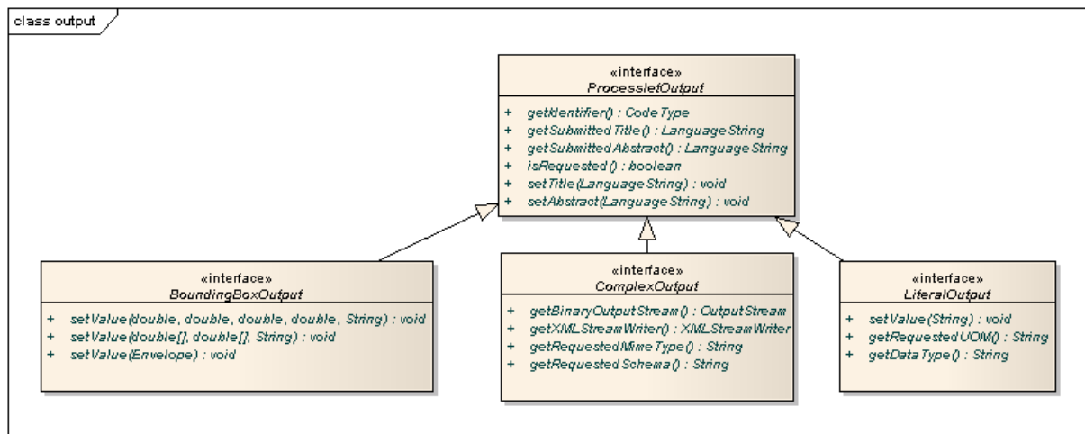
Figure 15.3: ProcessletOutput interface and sub types for each parameter type
