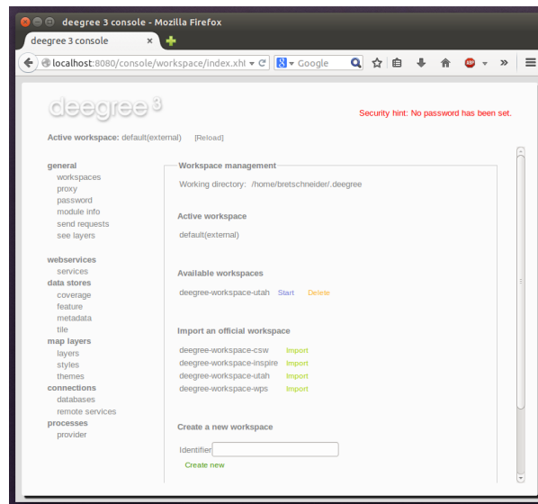
Figure 3.3: Downloaded, but inactive workspace
