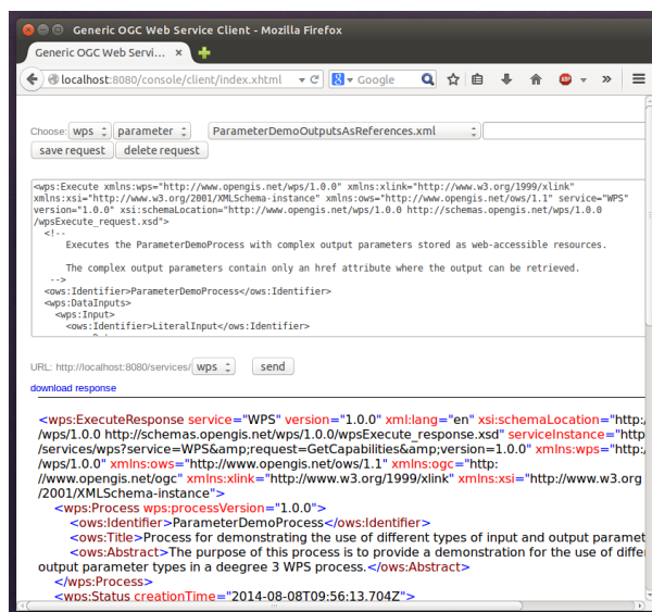
Figure 3.28: Example requests for the ParameterDemo process
