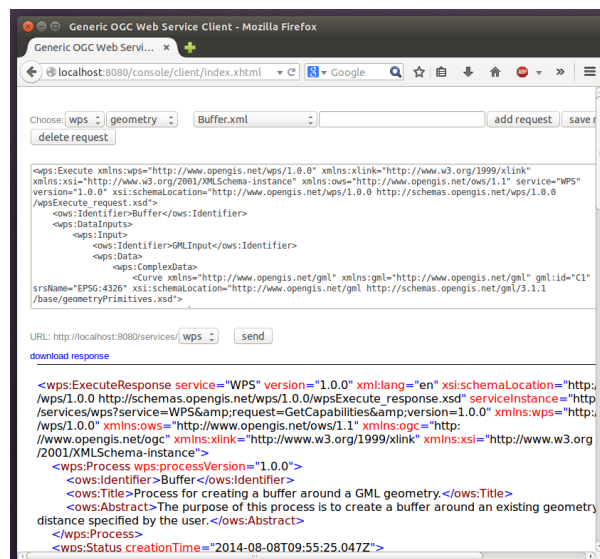
Figure 3.26: WPS response is displayed
