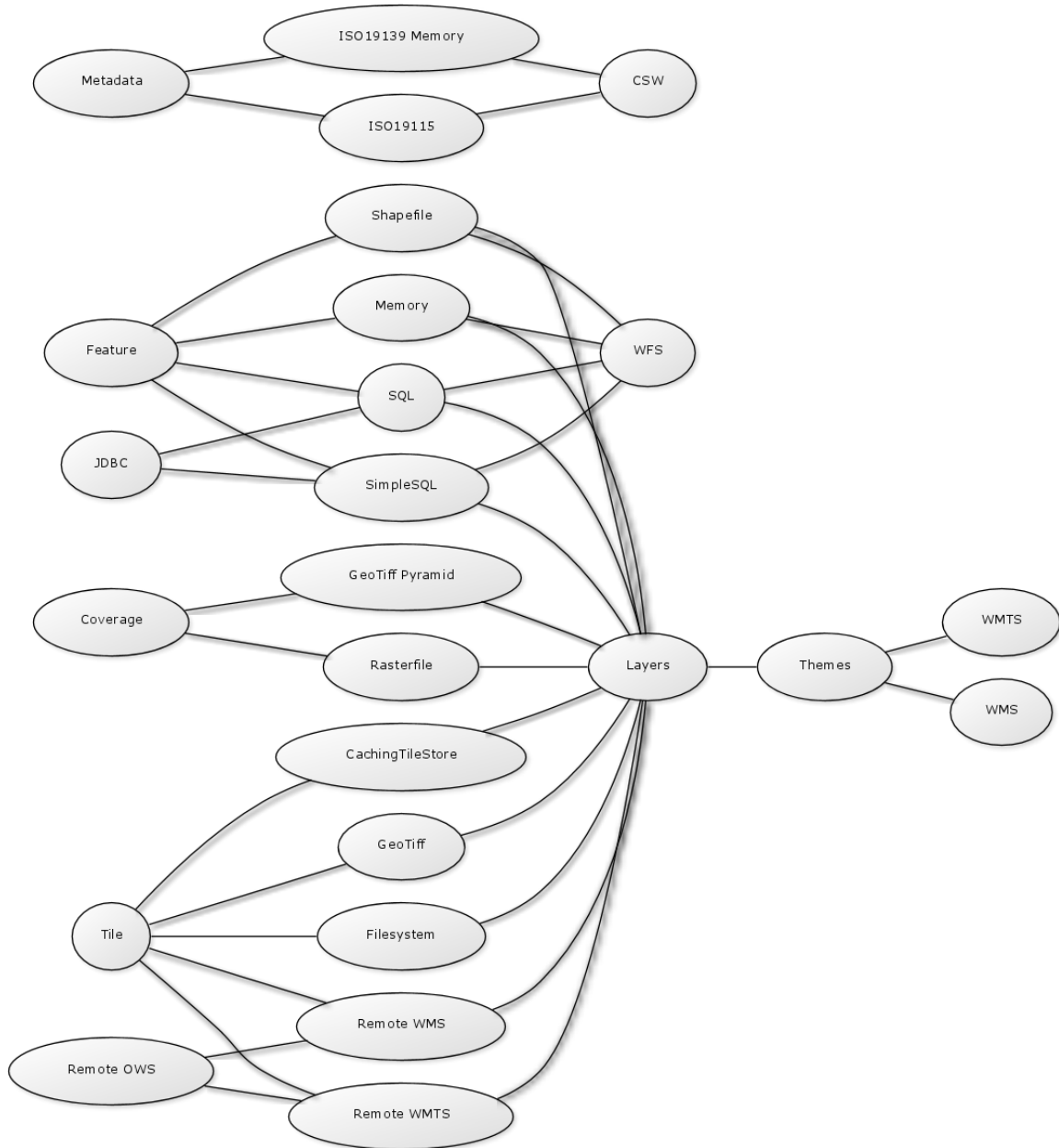
Figure 4.2: Workspace configuration dependencies
