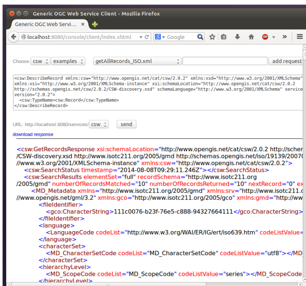
Figure 3.23: Other example CSW requests
