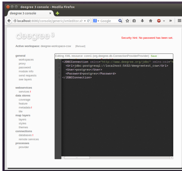
Figure 3.17: Editing the JDBC resource configuration file
