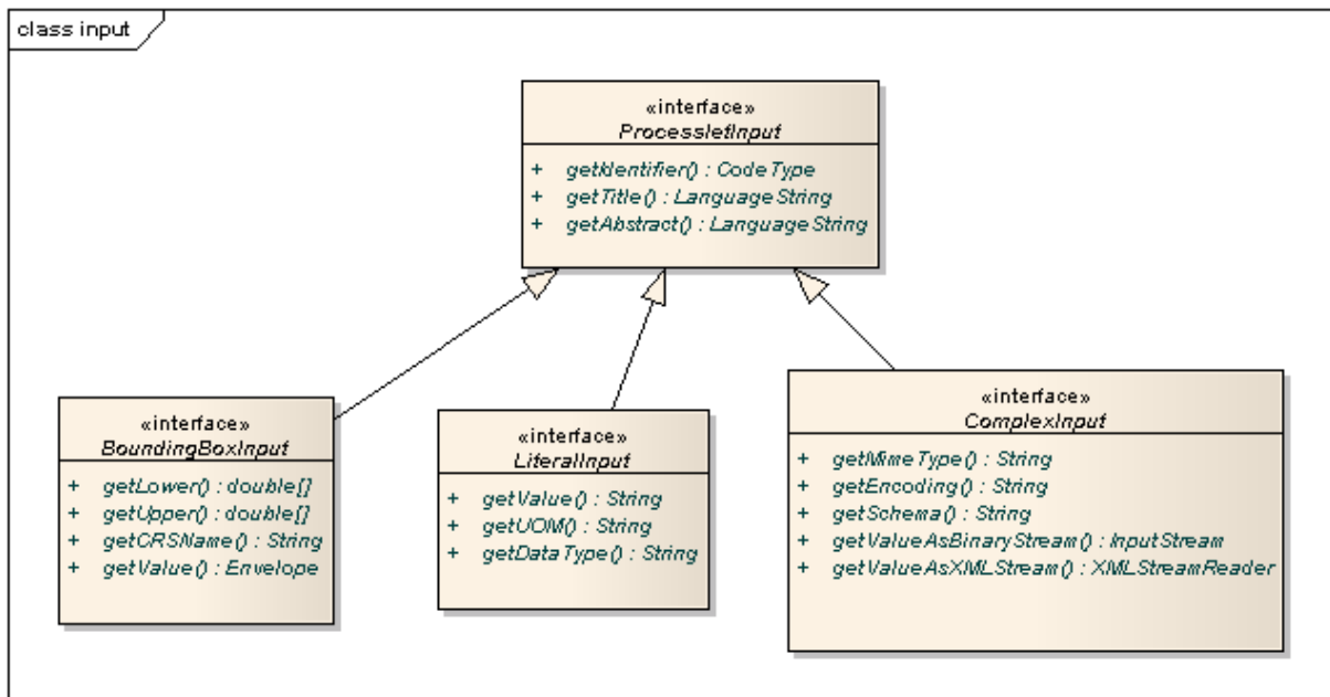
Figure 15.2: ProcessletInput interface and sub types for each parameter type
