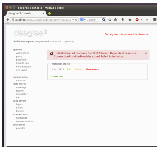
Figure 4.20: Error message
