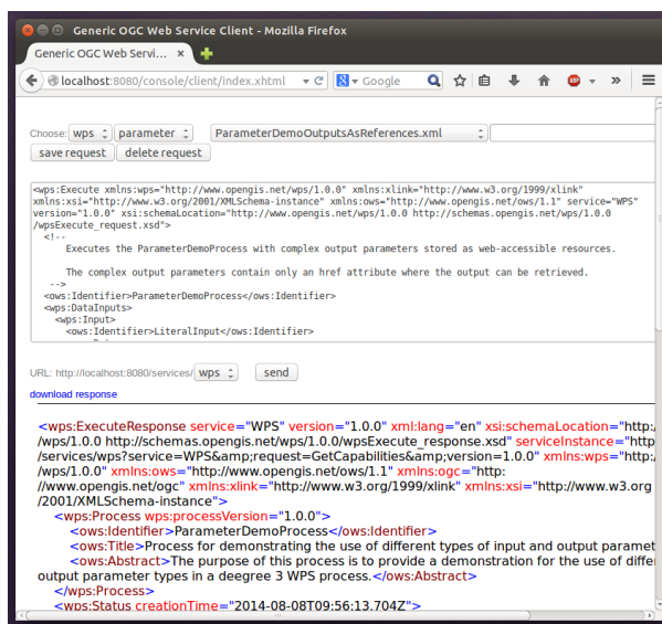
Figure 3.28: Example requests for the ParameterDemo process
