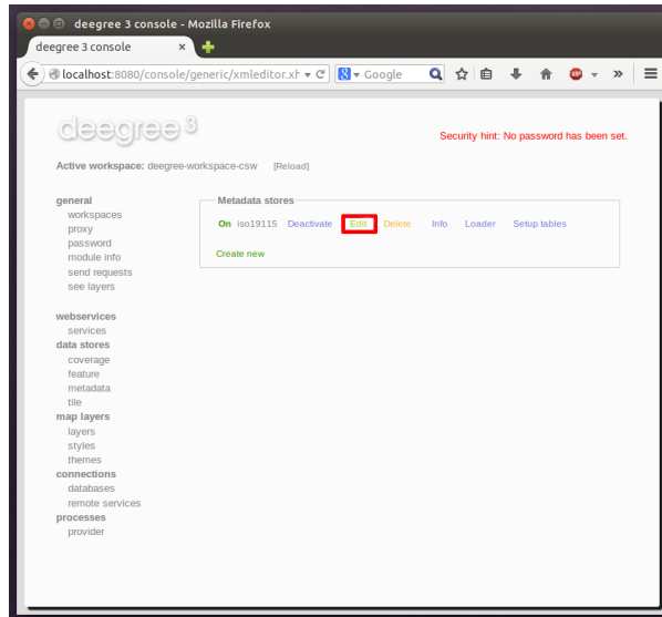
Figure 4.9: Edit action
