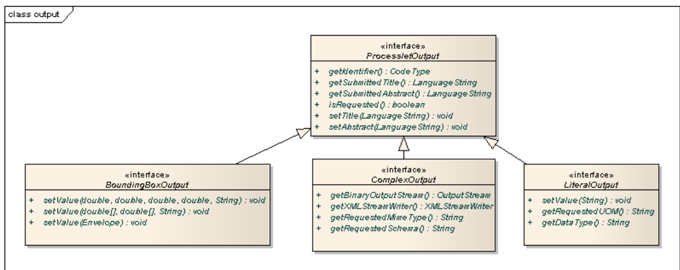
Figure 94. ProcessletOutput interface and sub types for each parameter type
