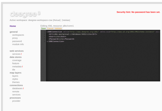
Figure 9. Editing the JDBC resource configuration file
