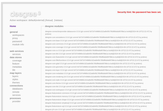
Figure 58. Displaying available JARs using the administration console
