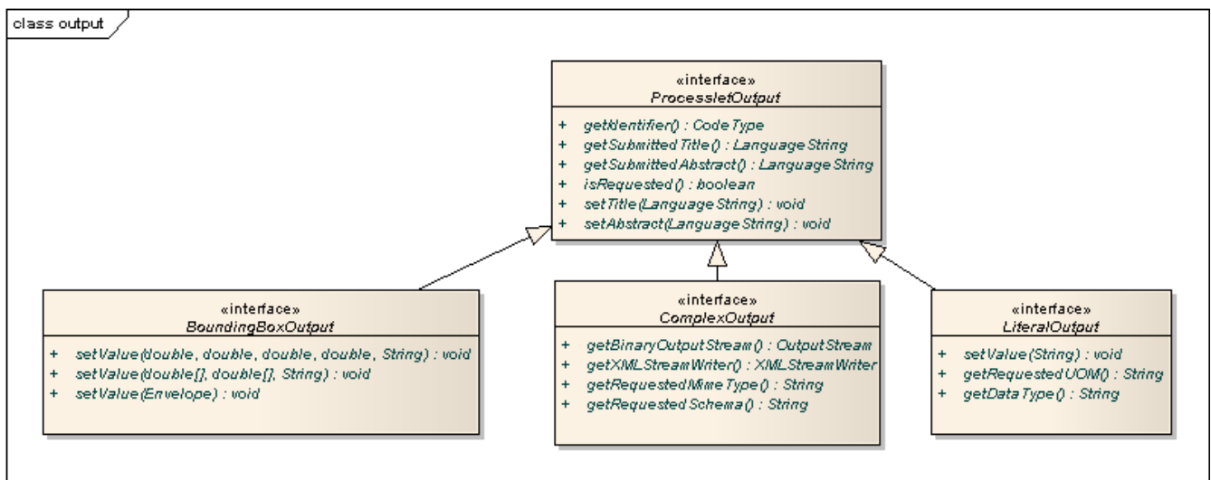
Figure 57. ProcessletOutput interface and sub types for each parameter type
